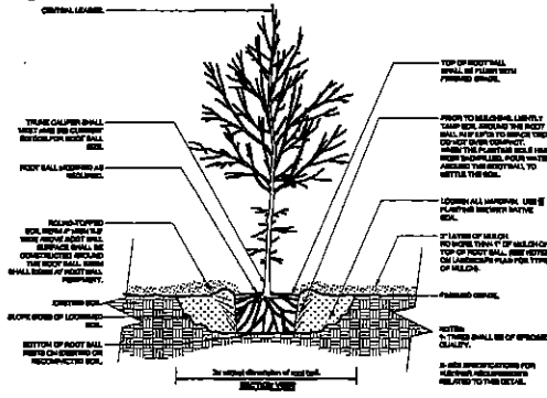
3 TREE PLANTING NOT TO SCALE
